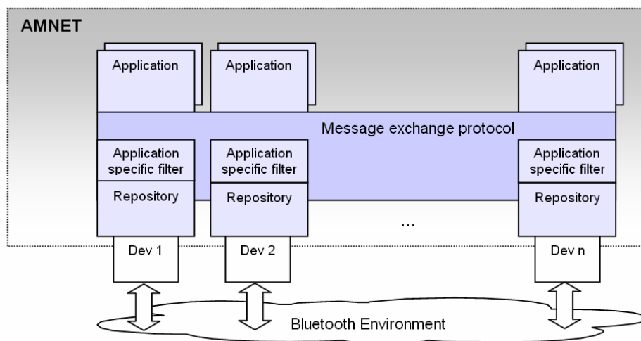
Figure 1: AMNET- Architecture
